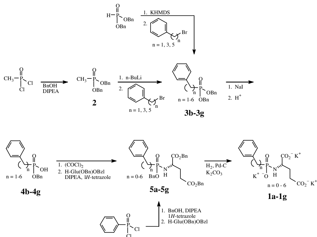
Scheme 1. Synthesis of phenylalkylphosphonamidate derivatives of glutamic acid.
