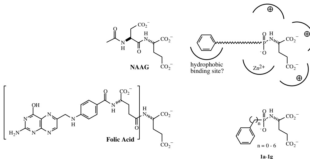
Figure 1. Substrates of PSMA and a binding model for a hydrophobic probing inhibitor.
