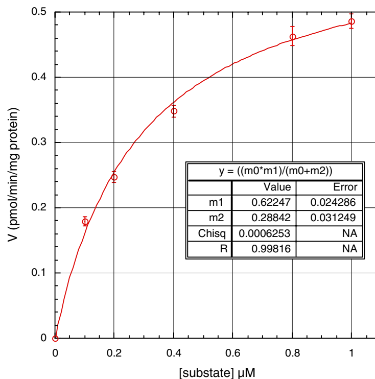
Figure 4. Kinetics of PSMA with PABG \gamma G 7.
