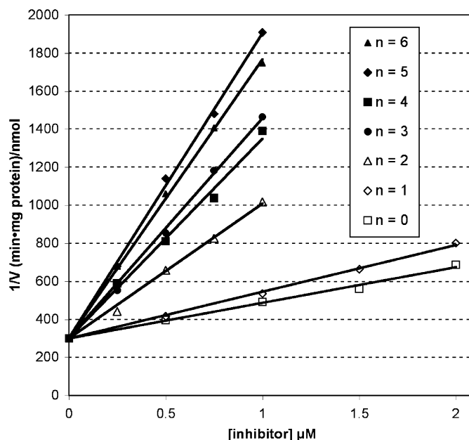
Figure 5. Dixon analysis of phosphonamides 1a–g . (*Each point represents the average of triplicate determinations.)
