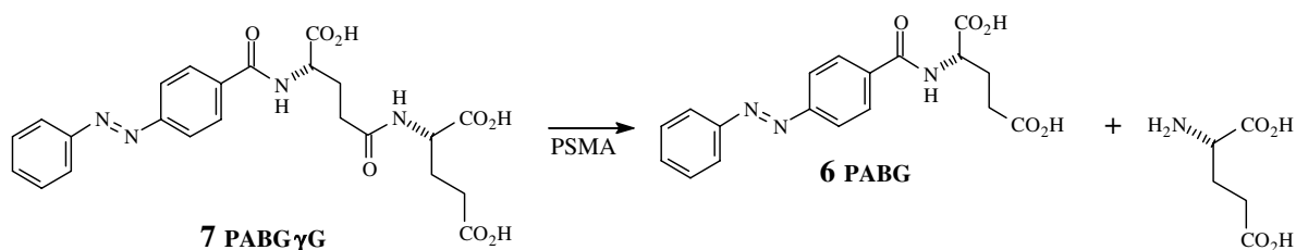
Figure 2. PSMA-mediated hydrolysis of PABG \gamma G to PABG.
