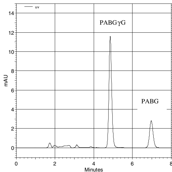
Figure 3. HPLC chromatogram of PABG \gamma G and PABG. Lichrosphere C18 150 \times 4.6 mm 5 \mu m; 40% ACN, 60% phosphate (pH 2.0, 25 mM) 1.0 mL/min; 325 nm.
